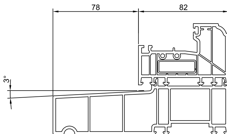
P90201 Storm 2 56mm Outer frame P90120 Storm 2 160mm x 45mm Sill
