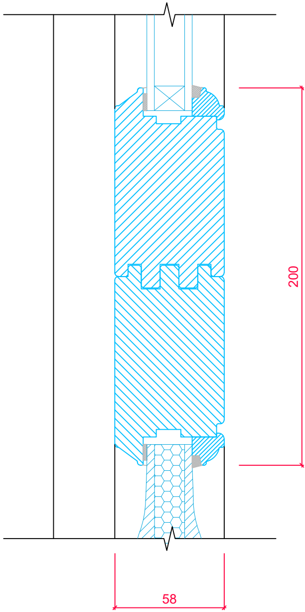
FRAME CROSS SECTION 'A-A'
