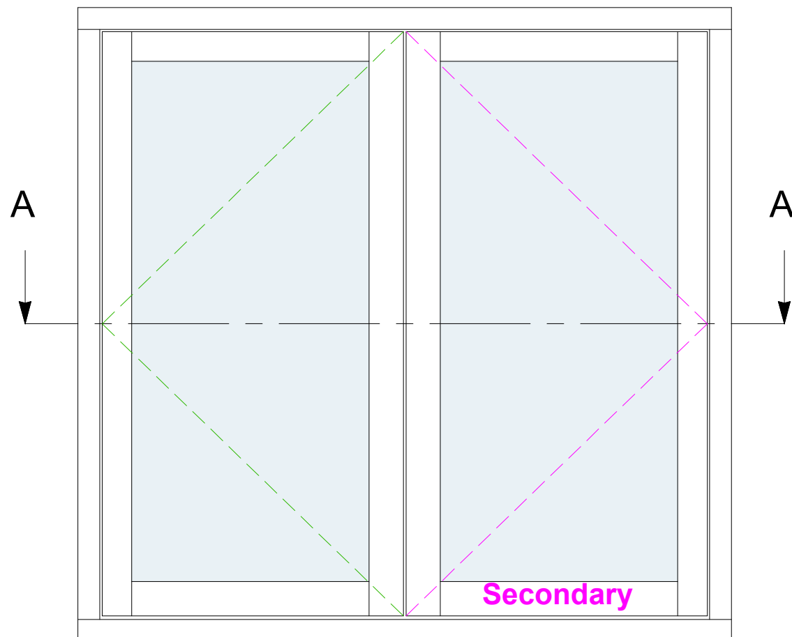
TYPICAL CASEMENT LAYOUT (SCALE 1:10)
