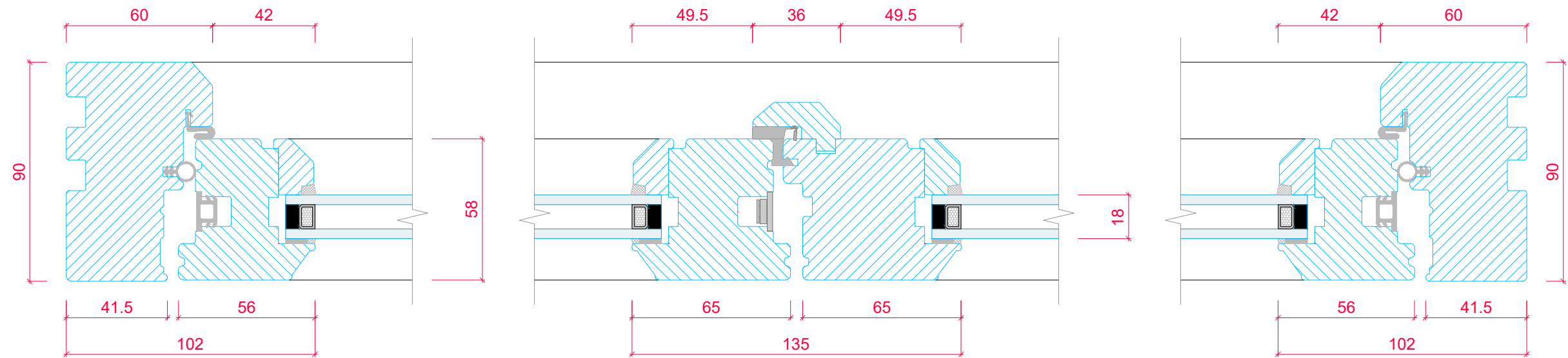
CASEMENT CROSS SECTION 'A-A' (SCALE 1:2)
