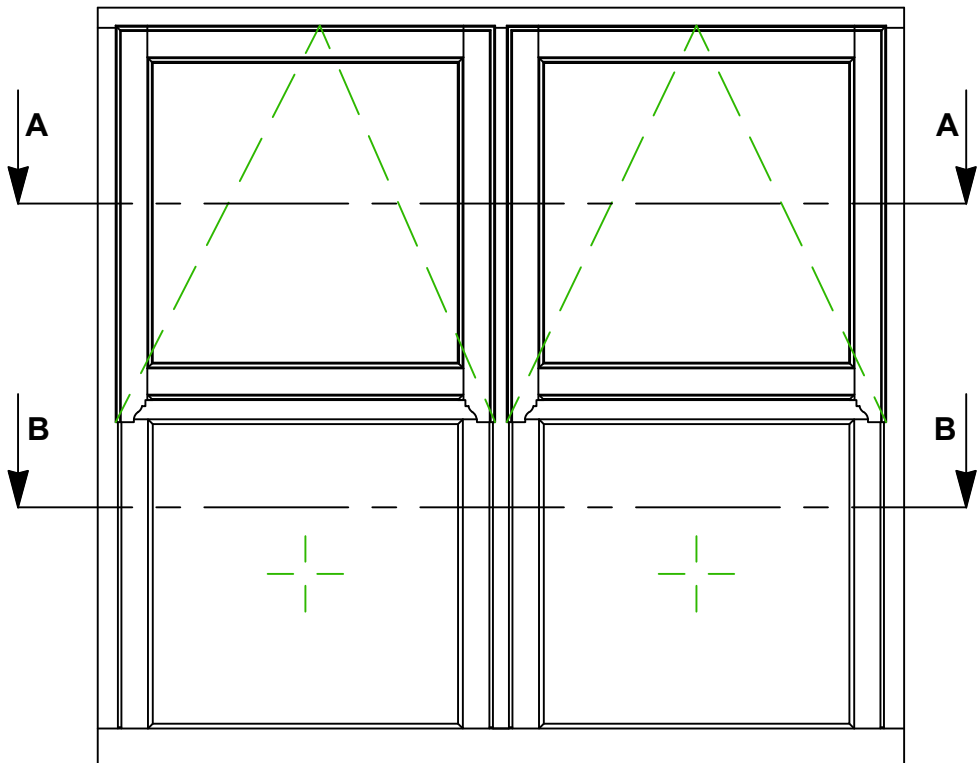
TYPICAL MOCK SASH LAYOUT
