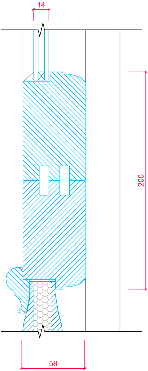
FRAME CROSS SECTION 'A-A'
