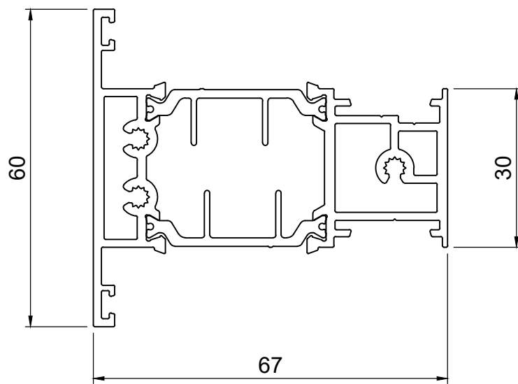
60mm Transom / Mullion
