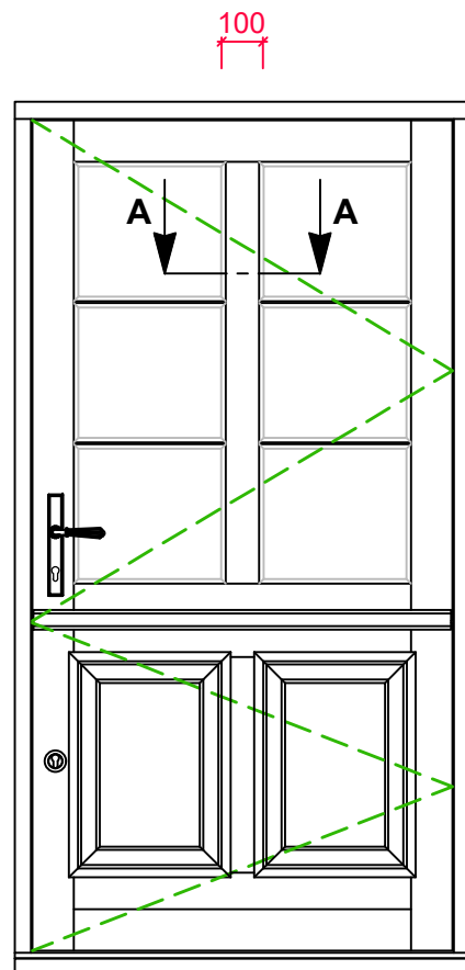
TYPICAL FRAME LAYOUT
