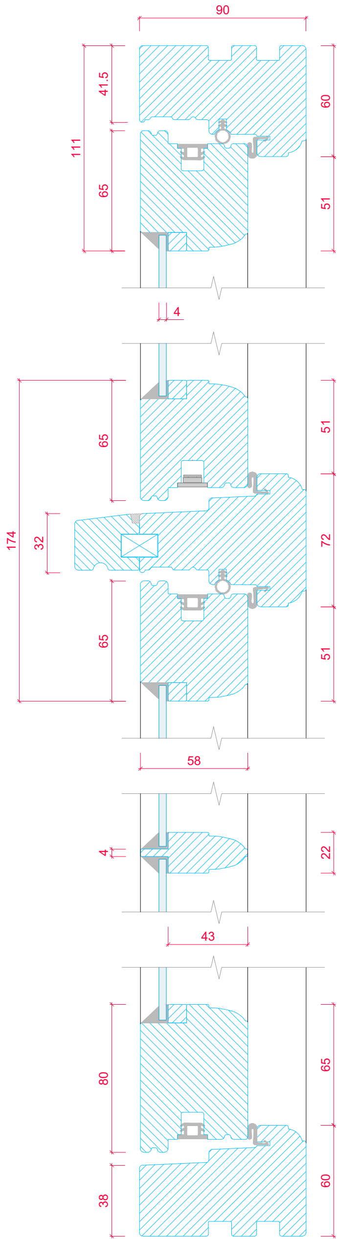
CASEMENT CROSS SECTION 'A-A' (SCALE 1:2)
