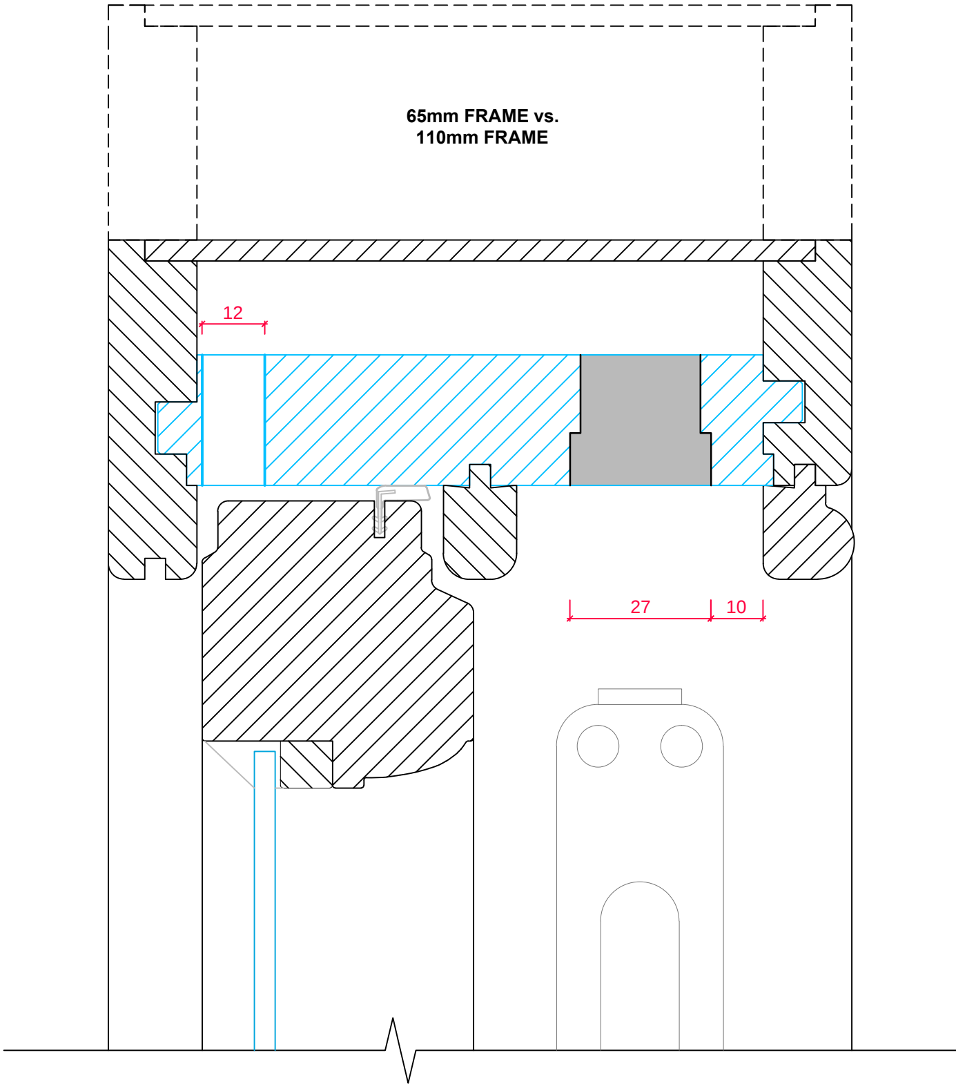
TRICKLE VENT IN HEAD OF FRAME AVAILABLE IN 65mm AND 110mm FRAME WIDTHS UNAVAILABLE IN SASH TOP RAIL
